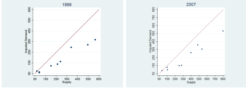
Figure 4: A Cross-Section Test of Production in the HOV Theory
